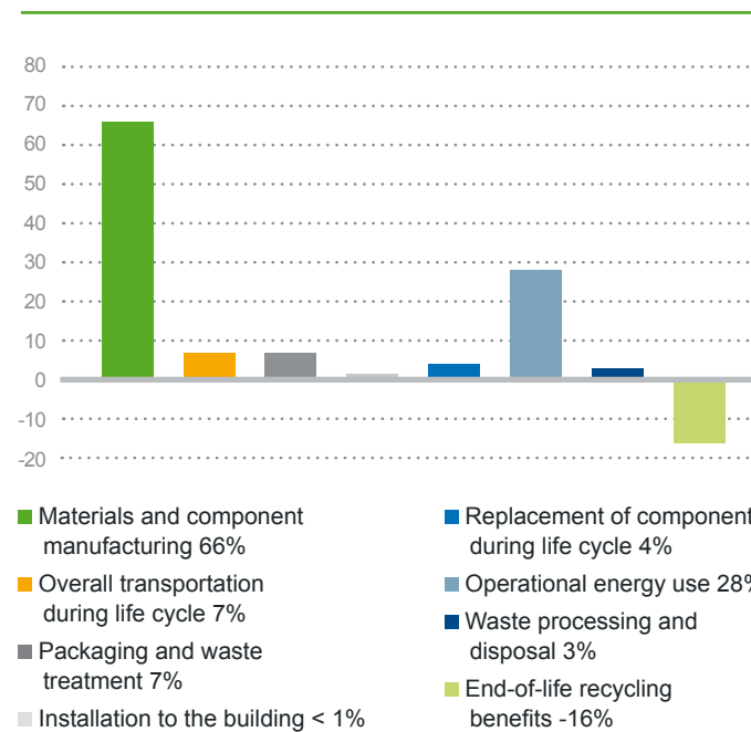
Life cycle carbon footprint of KONE MonoSpace® 700 DX elevator is approximately 24 tCO 2 e
